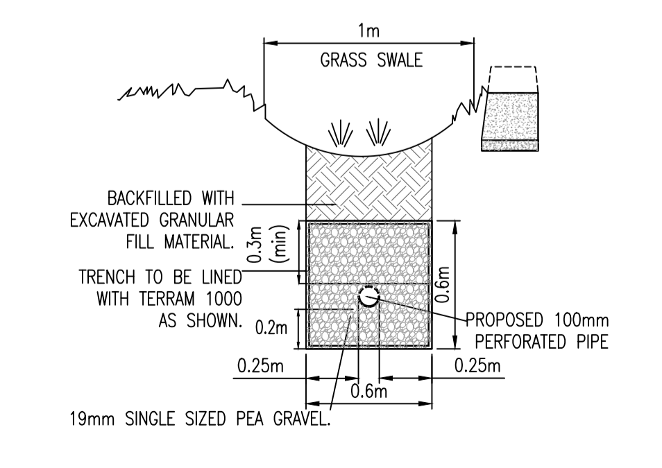
TYPICAL SECTION THROUGH PROPOSED SWALE
