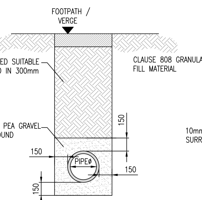
TYPICAL PIPE BEDDING DETAILS NON TRAFFICKED AREAS
