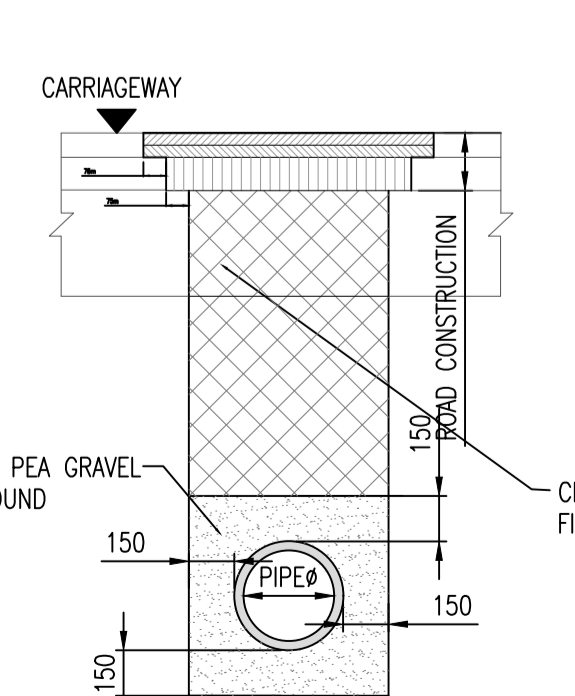
TYPICAL PIPE BEDDING AND REINSTATEMENT DETAILS
