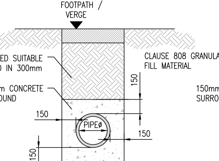
TYPICAL PIPE BEDDING DETAILS NON TRAFFICKED AREAS LESS THAN 900mm TO PIPE CROWN
