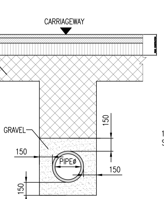
TYPICAL PIPE BEDDING DETAILS TRAFFICKED AREAS
